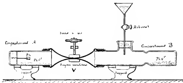
FIG. 51.— Apparatus of Gustave Le Bon and Martin, used for determining the part played by water vapour in the phosphorescence of phosphorus. —The two compartments A and B being supplied with anhydrous phosphoric acid, phosphorus is introduced into A, then A and B are separated by tightening the screw V. The phosphorus absorbs the oxygen of A, shines and then becomes extinguished. The screw V is then loosened and the dry air from B penetrates into A. One observes only a very slight phosphorescence, confined to the surface of the piece of phosphorus. If then, by means of the funnel represented in the figure, a drop of water is allowed to fall into B, the small quantity of vapour it emits is enough to render the phosphorus much more brilliant and there will form round it a luminous cloud. Water vapour therefore plays a manifest part in phosphorescence.
