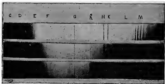
FIG. 43.— Photographs showing the disappearance of the solar ultra-violet on certain days caused by unknown influences. —The upper band represents an ordinary solar spectrum extending to the borders of the N ray. The band beneath it shows the disappearance of the solar ultra-violet starting from the L ray, notwithstanding the prolongation of the exposure. The lower band represents the total disappearance of the ultra-violet when the spectrum is photographed through a transparent solution of sulphate of quinine.
